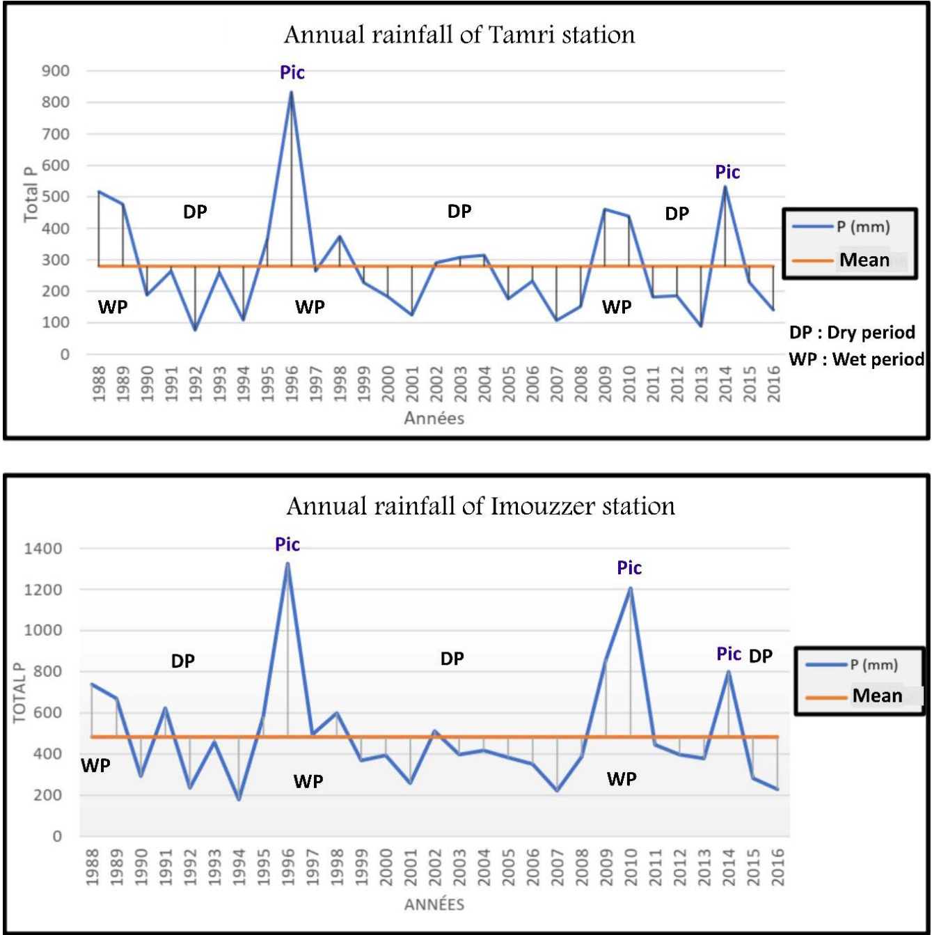
Figure 9. Diagrams of the annual rainfall recorded in two climatic stations. WP: Wet Period, DP: Dry Period. Source: own elaboration based on hydraulic basin agency Souss Massa , 2017.
