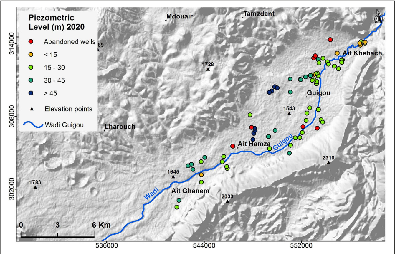
Figure 4. Distribution of the piezometric level in the Guigou depression (measurements conducted using a piezo-metric probe in March 2020). Source: own elaboration based on piezometric measurements conducted in the Guigou Depression in March 2020.
