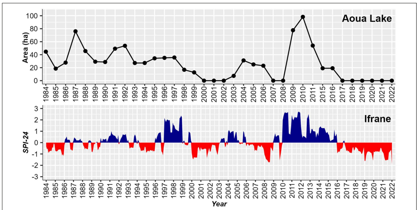
Figure 8. Comparison between the lake water area and the 24-month SPI at the Ifrane station between 1984 and 2022. Source: own elaboration based on processing of rainfall data derived from the Sebou Hydraulic Basin Agency and Landsat TM, OLI, and OLI-2 satellite images.
