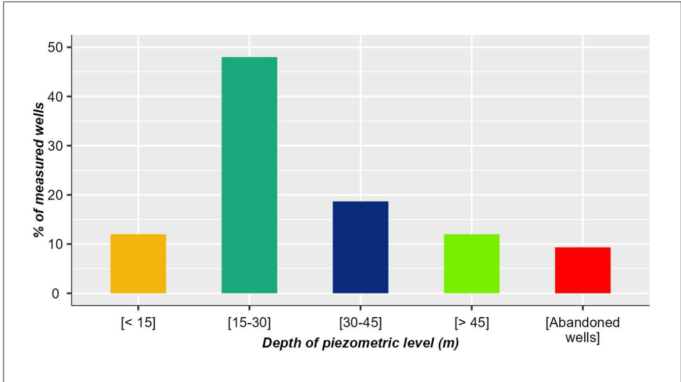
Figure 5. Piezometric level classes (m) in the Guigou depression in March 2020. Source: own elaboration based on piezometric measurements conducted in the Guigou Depression in March 2020.
