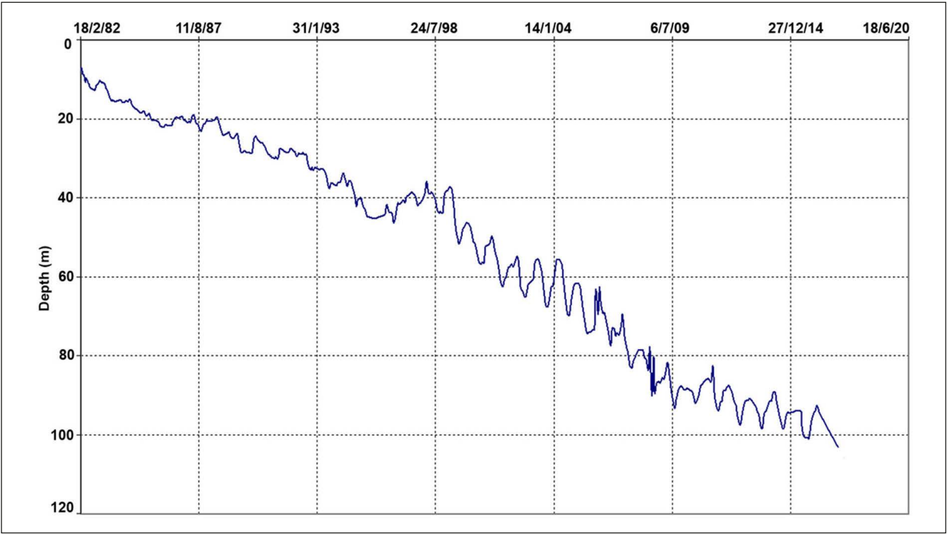
Figure 3. Evolution of the piezometric level in the Fez Meknes aquifer between 1982 and 2017. Source: own elaboration based on Sebou Hydraulic Basin Agency, Data accessed, January 31, 2024.
